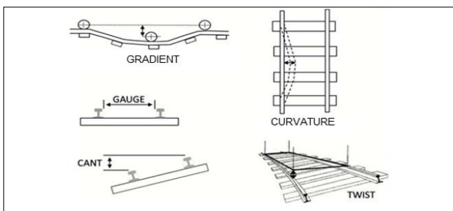
Track measurement parameters: gradient, gauge, cant, curvature and twist
