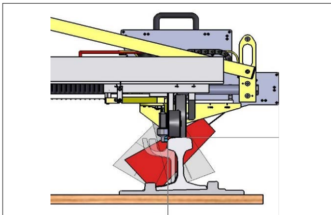
3 lasers per rail to scan in data on the rail head of grooved or flange rails
