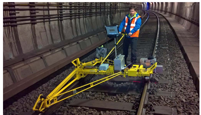
Measuring the track geometry using KRAB trolley
